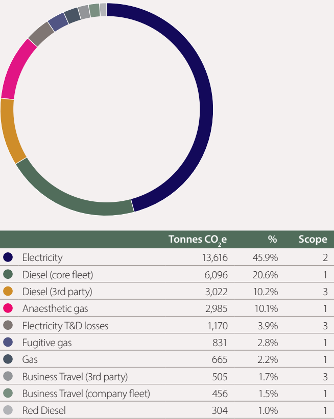
Carbon emissions breakdown by source 2020/21
